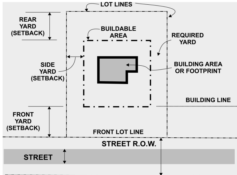
Figure 2-4 BUILDABLE AREA
